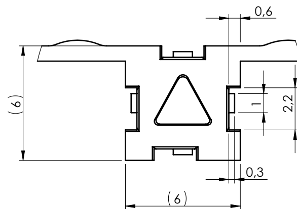
DETAIL D SCALE 5 : 1
