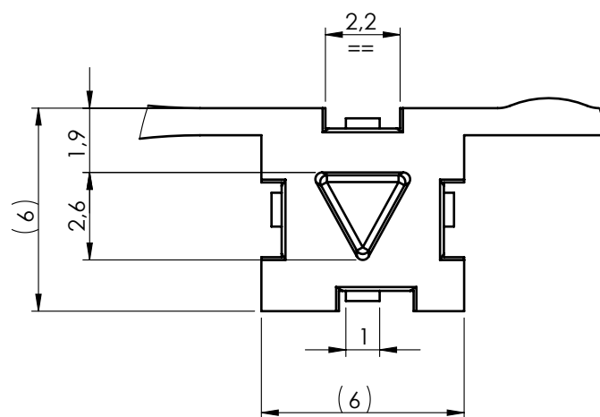
DETAIL C SCALE 5 : 1
