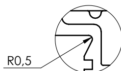
DETAIL A SCALE 2 : 1
