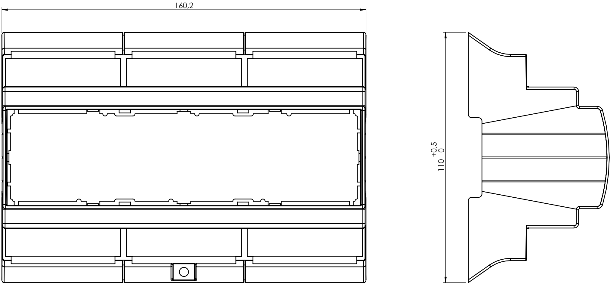
BODY ENCLOSURE
