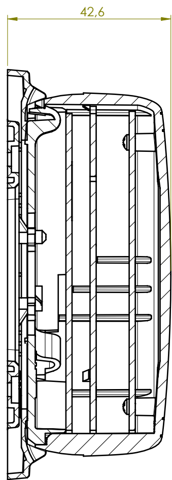
SECTION F-F
