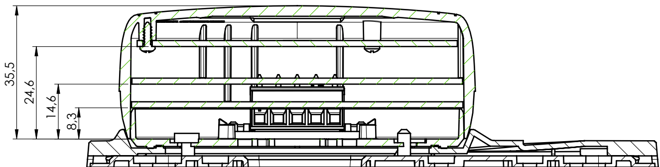
SECTION G-G
