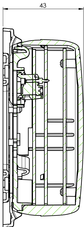
SECTION F-F
